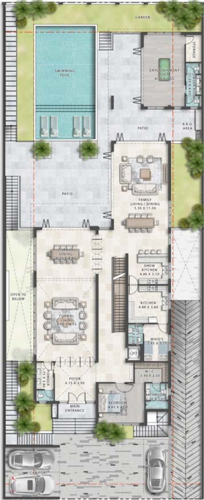
GROUND FLOOR
